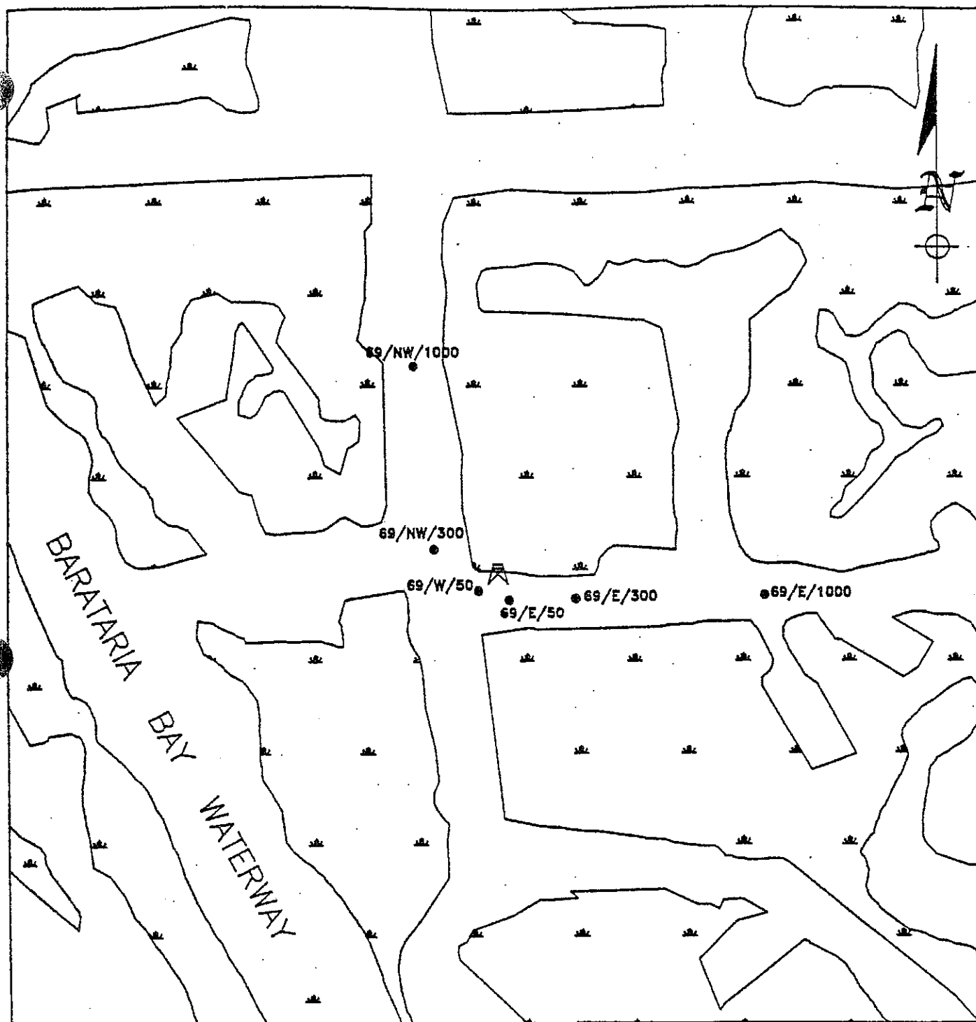
FIGURE 16 STATION 69 CF #10 TANK BATTERY #8 SAMPLE LOCATIONS LAFITTE FIELD
