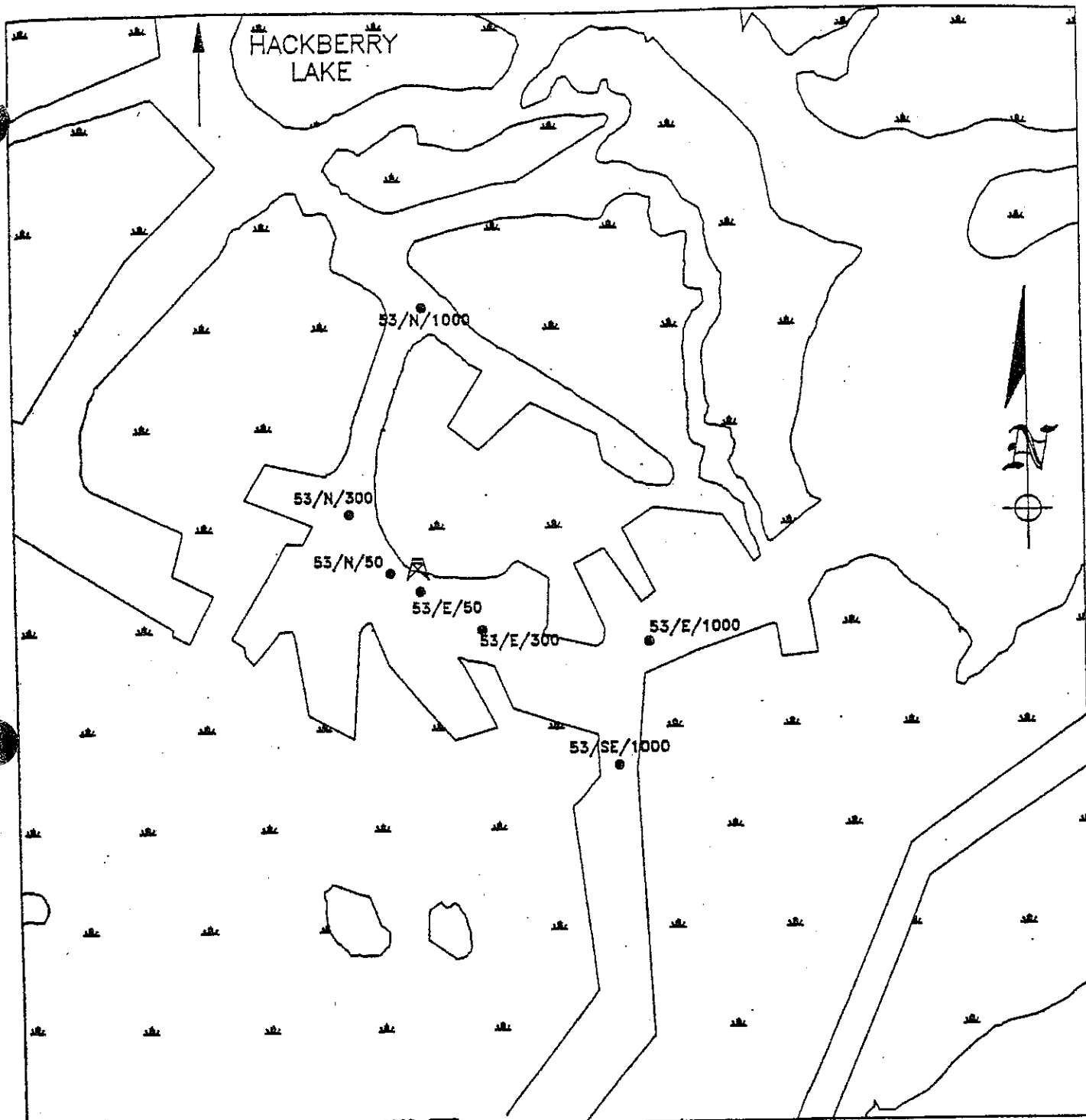
FIGURE 8 STATION 53 CF #6 TANK BATTERY #7 SAMPLE LOCATIONS DOG LAKE FIELD
