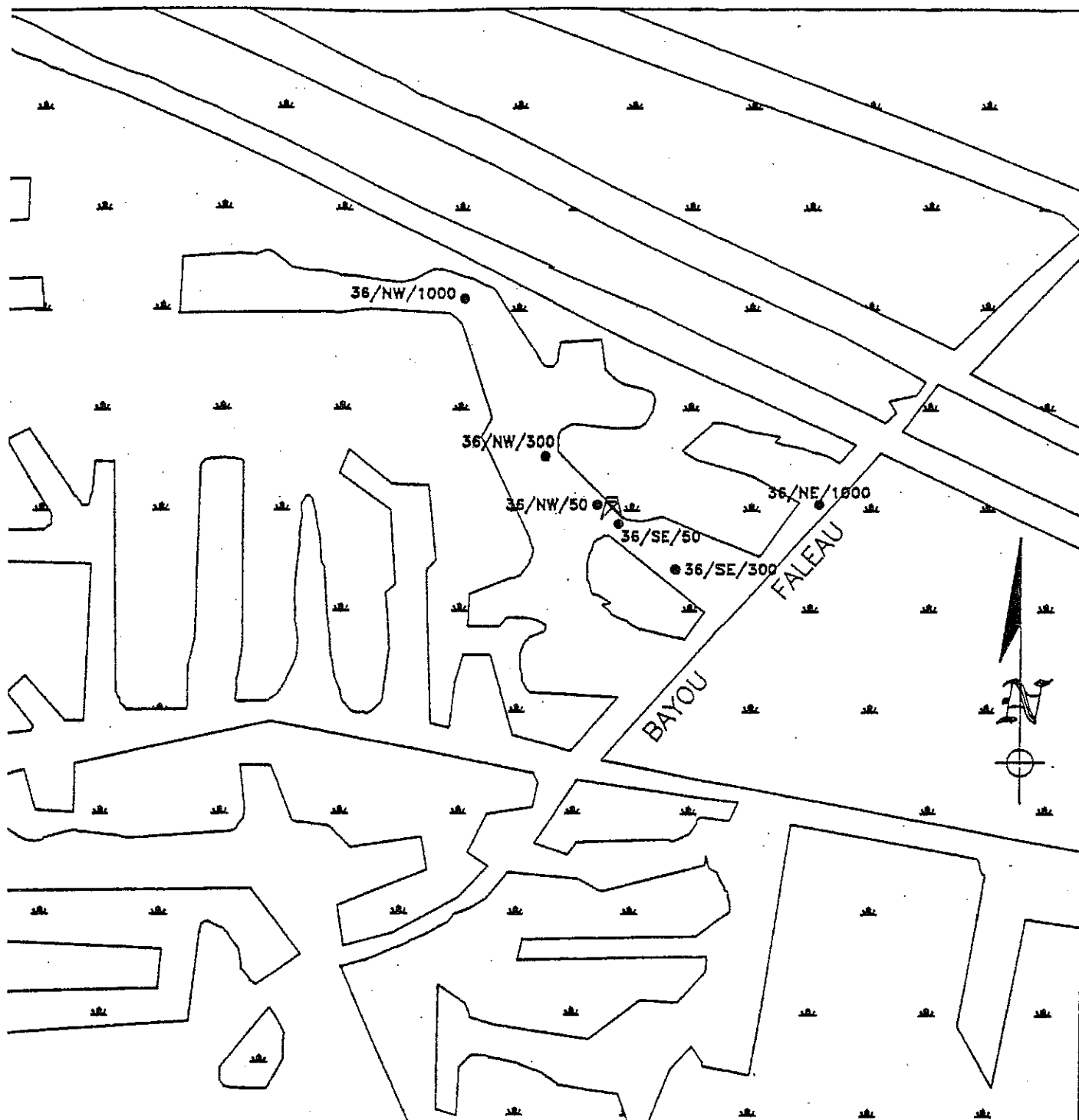
FIGURE 7 STATION 36 TANK BATTERY #10 SAMPLE LOCATIONS GOLDEN MEADOW FIELD
