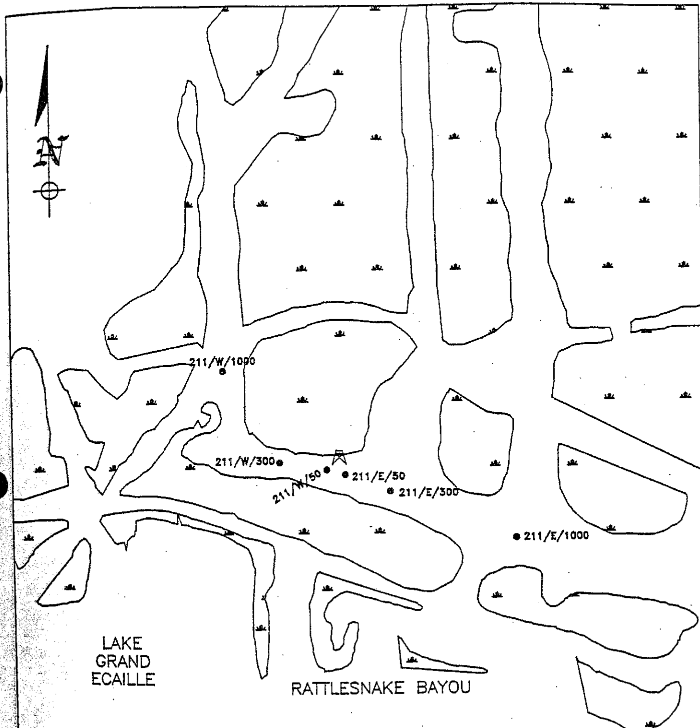
FIGURE 30 STATION 211 CENTRAL TANK BATTERY SAMPLE LOCATIONS LAKE WASHINGTON FIELD
