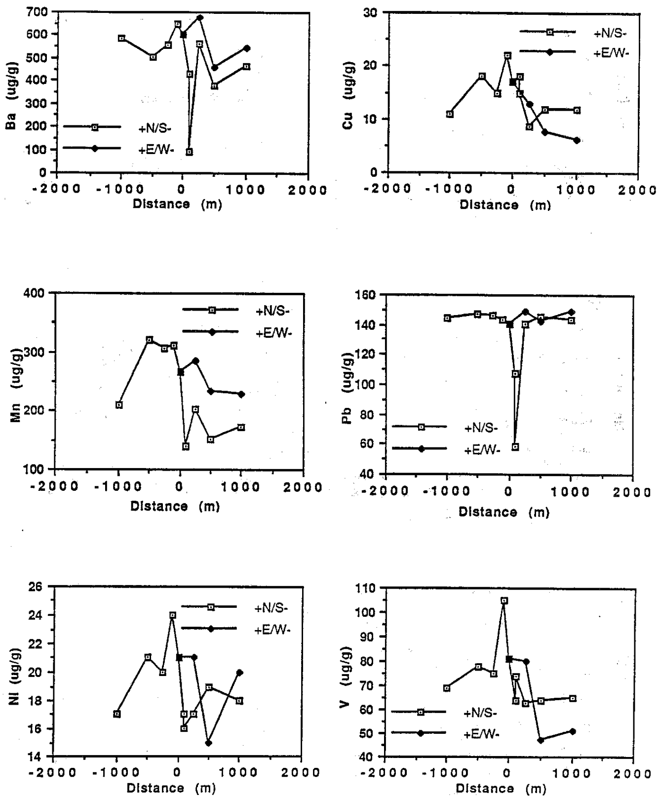
Figure 8.20. Spatial distribution of selected trace metals for Golden Meadow primary site sediments.
